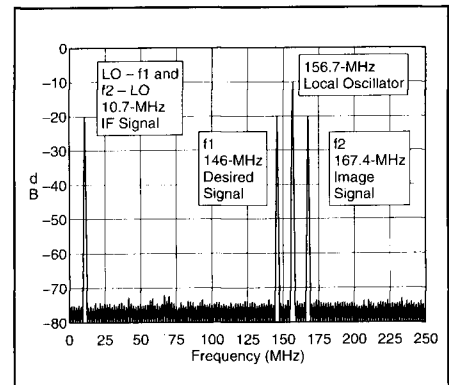
Figure 4—A superheterodyne receiver can respond to signals other than the desired signal. If the RF selectivity of the receiver is inadequate (poor image rejection), the receiver could hear the signal on 167.4 MHz in addition to the desired signal on 146 MHz.
