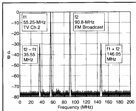
Figure 2—Here, f1 (55.25 MHz) and f2 (90.8 MHz) are present at the input of a VHF receiver, they may generate an interfering signal ( f1 + f2 ) on 146.05 MHz.
