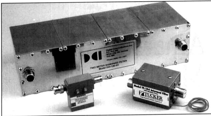
Figure 5—Two of the three shown are band-pass filters (discussed here). One of them is a notch filter (discussed later). All three are commercial.
