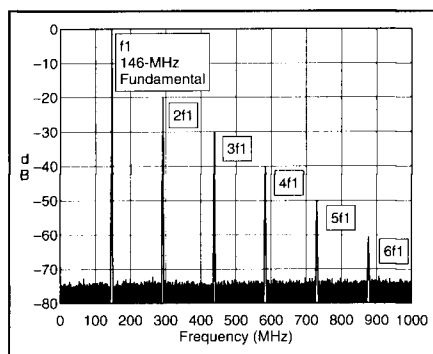
Figure 1—This 146-MHz signal contains harmonics that extend well into the UHF range.
