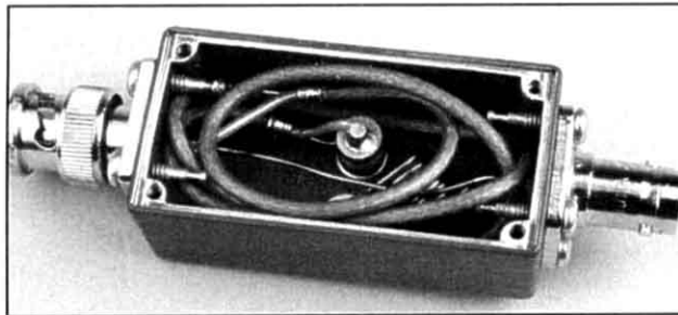
Figure A—This simple notch filter is easy to tune and uses available components.
