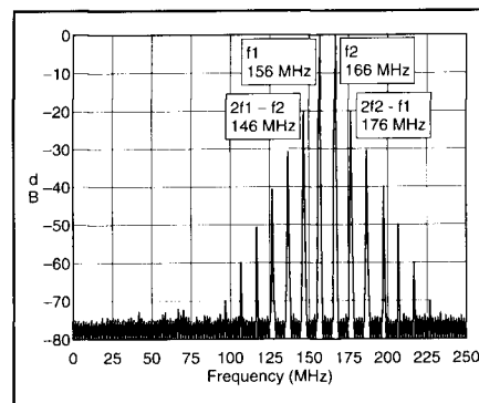
Figure 3—These pager frequencies can intermodulate to form a product in the amateur 2-meter band. If there are many pagers on different frequencies in the same area, the result can be interference across the band. This actually occurs in some major cities. This graph shows third- and higher odd-order products.
