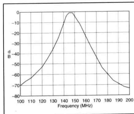
Figure 6—The frequency response of a typical band-pass filter. This filter's passband centers near 147 MHz. Its 3-dB bandwidth is about 7 MHz (143 to 150 MHz).
